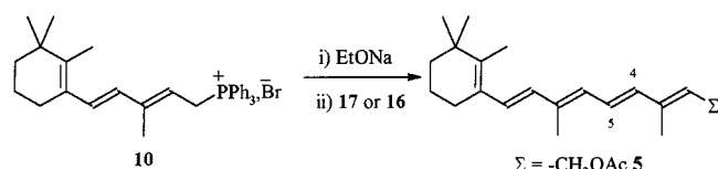
Scheme 4. \text{C}_{15} + \text{C}_5 coupling
