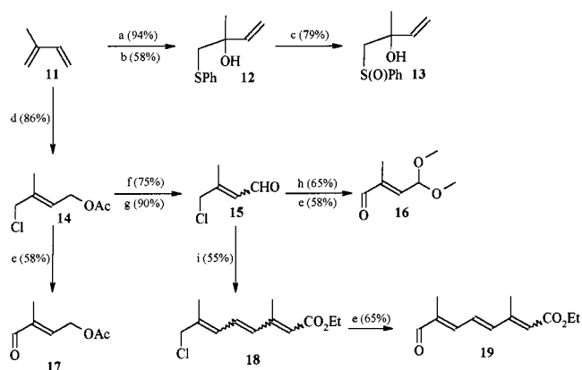
Scheme 6. Preparation of linear aldehydic units 16 , 17 and 18 ; reagents and conditions: (a) NBS, acetone/H 2 O; (b) PhSNa, DMF; (c) NaIO 4 , t BuOH/H 2 O; (d) t BuOCl, AcOH then CuSO 4 , H 2 SO 4 ; (e) DMSO, K 2 HPO 4 /KH 2 PO 4 , NaBr, 80°C; (f) Na 2 CO 3 , MeOH/H 2 O; (g) PCC, CH 2 Cl 2 ; (h) HC(OCH 3 ) 3 , MeOH, APTS; (i) Ph 3 P=CHC(CH 3 )=CHCO 2 Et then I 2
