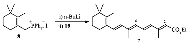
Scheme 5. \text{C}_{10} + \text{C}_{10} coupling
