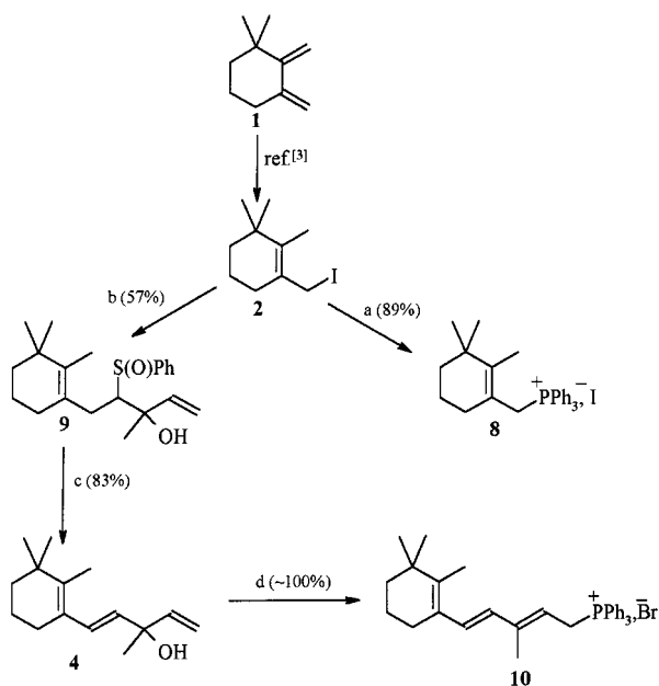
Scheme 3. Preparation of phosphonium salts 8 and 10 ; reagents and conditions: (a) \text{PPh}_3 , \text{Et}_2\text{O} ; (b) 13 , n\text{BuLi} (2 equiv.), THF, -78^\circ\text{C} ; (c) \text{K}_2\text{CO}_3 , toluene, reflux; (d) \text{PPh}_3/\text{HBr} , MeOH
