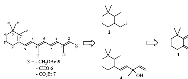
Scheme 2. Retrosynthetic analysis for the obtention of "iso"-retinoids 5–7
